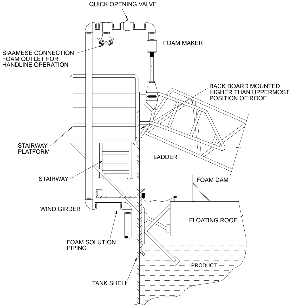
SEAL AREA PROTECTION USING A FOAM MAKER OR HANDLINE NOZZLE FROM LADDER AREA
